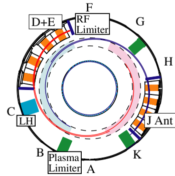
Fig. 1. Top view schematic showing the location of the antennas (D + E and J), plasma limiters (green), RF limiter (blue ~1 cm behind plasma limiter) and example of field lines mapped from each antenna. Note that these field lines map to toroidally distinct locations and the dashed circles mark the top of the outer divertor. (For interpretation of the references in colour in this figure legend, the reader is referred to the web version of this article.)
