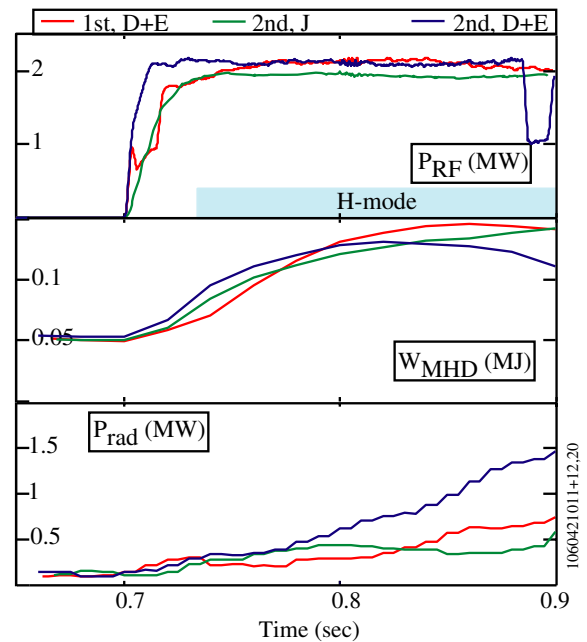
Fig. 3. Comparison of stored energy and radiated power for control and test discharges. The red curve is representative of first discharge post boronization with D + E antenna and green is second discharge heated by J antenna. This discharge has nearly identical response as first and the second discharge heated by D + E shows its typical degradation and increase radiation. (For interpretation of the references in colour in this figure legend, the reader is referred to the web version of this article.)
