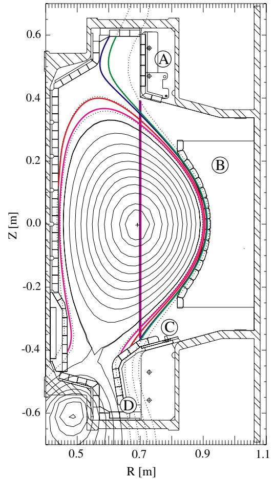
Fig. 2. Poloidal cross section showing tile groups: (A) gusset; (B) plasma limiter (RF limiter is \sim 1 cm further out in major radius); (C) top of outer divertor; and (D) strike point. A set of poloidal projections of field lines are shown. Note that the field lines ending on the outer shelf intersect near the EC resonance position during boronization where impurities were controlled more effectively.
