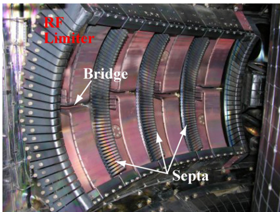
Fig. 5. J antenna with Faraday screen removed and septums installed. The RF limiter, septa, and bridge section of the current straps are indicated.
