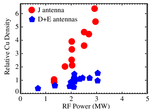
Fig. 7. Relative Cu density versus RF power for the J antenna with Faraday screen removed and D + E antennas.
