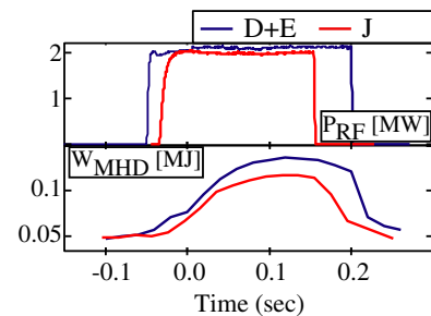
Fig. 6. Comparison of J antenna with Faraday screen removed and D + E antennas showing the degraded plasma performance.
